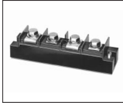
CM531213, CM531613 Dual SCR POW-R-BLOK™ Modules 130 Amperes/1200-1600 Volts
