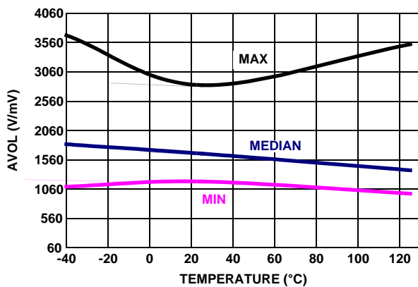
FIGURE 29. AVOL vs TEMPERATURE, V_+, V_- = \pm 2.5V, V_O = -2V \text{ TO } +2V, R_L = 100k
