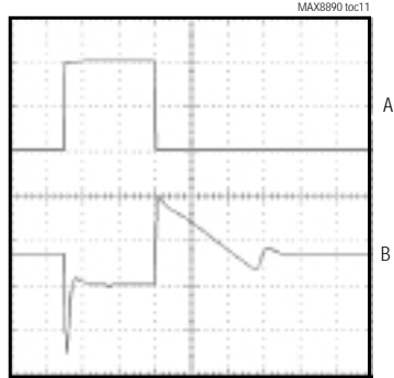
LOAD TRANSIENT NEAR DROPT
